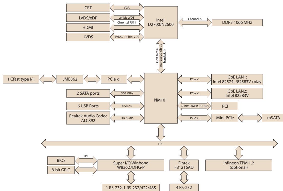
Figure 1.3 AIMB-214 Board Diagram
