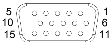
Figure 2.10 VGA Connector
