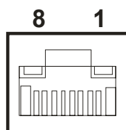
Figure 2.24 Ethernet Connector
