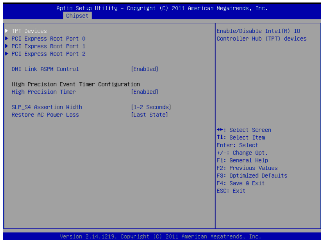
Figure 3.15 Chipset Setup
