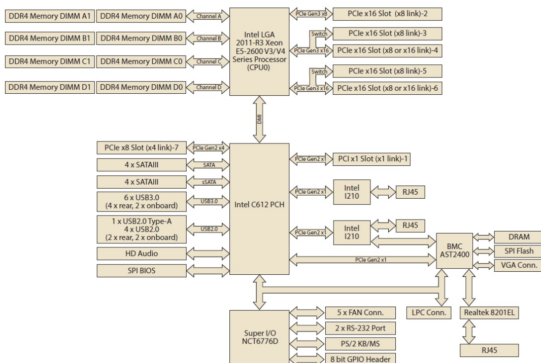
Figure 1.3 Block Diagram
