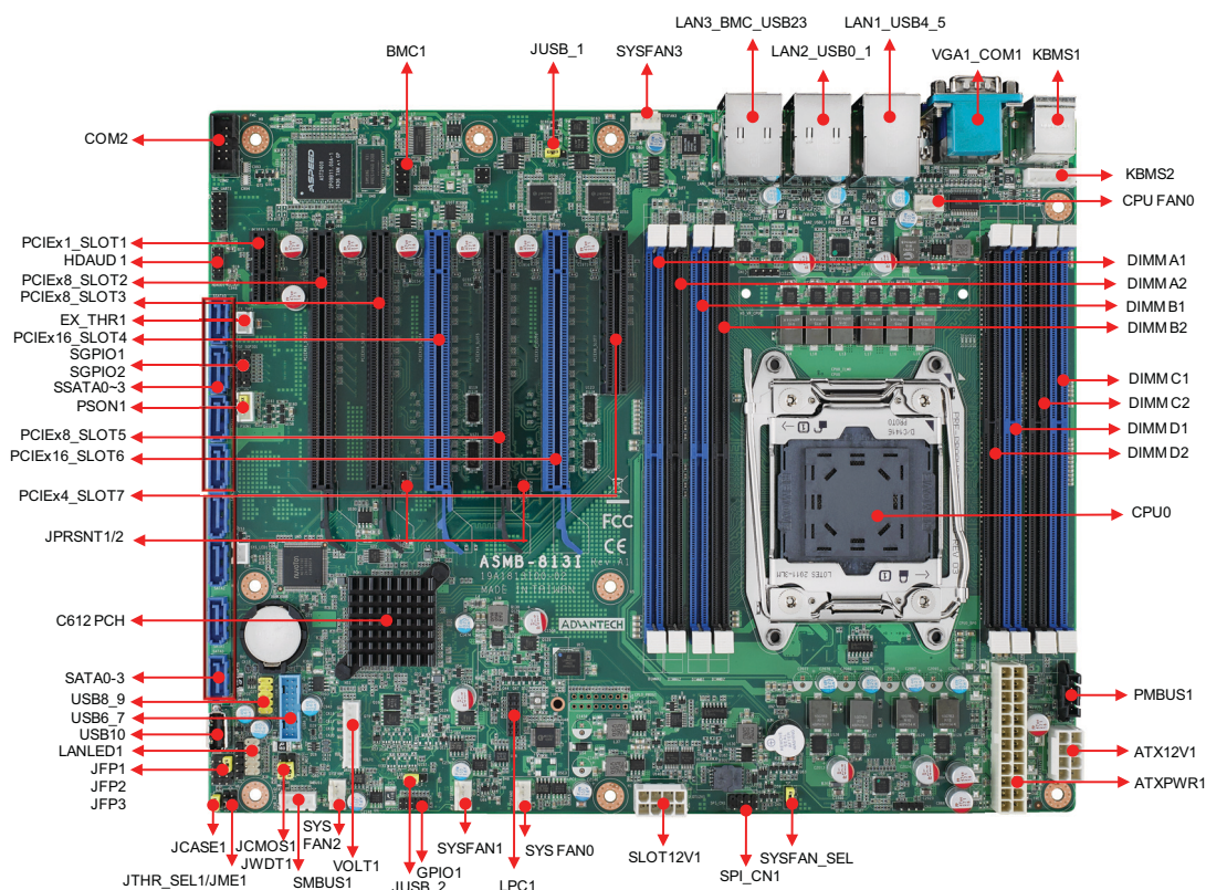
Figure 1.1 Board Layout
