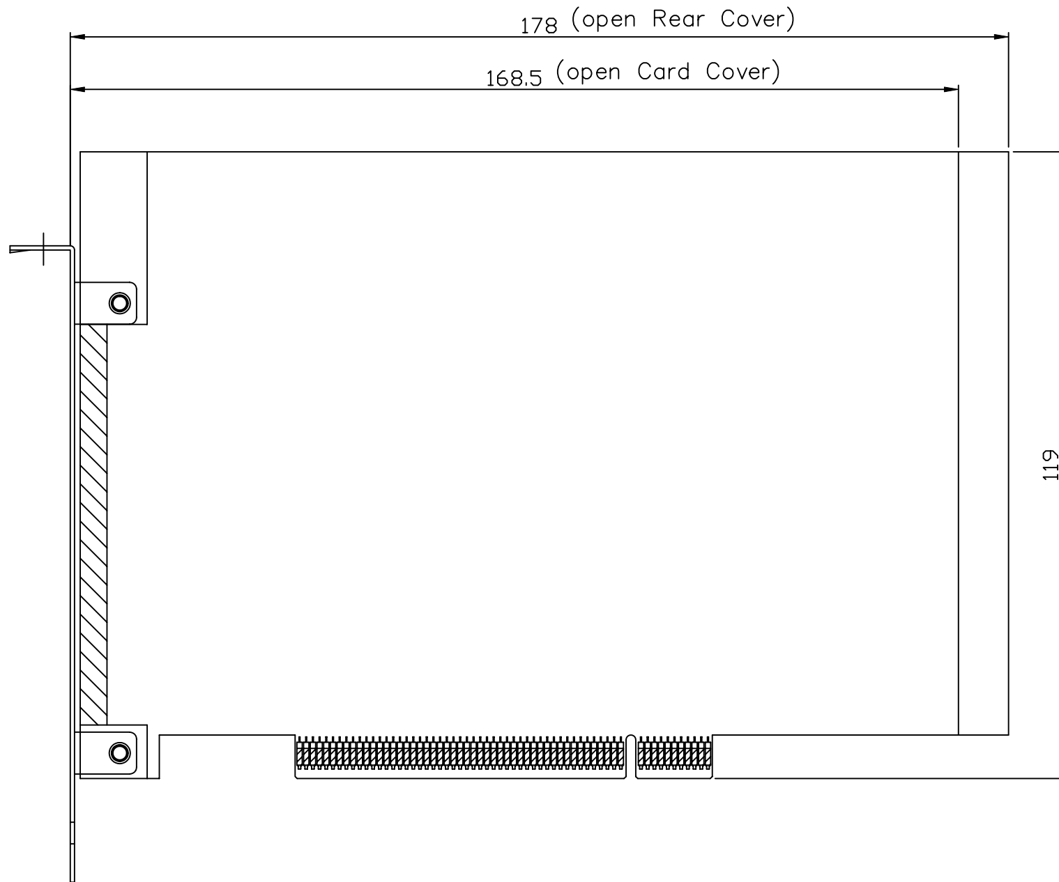
PPC-123 / 153 Add on card size
