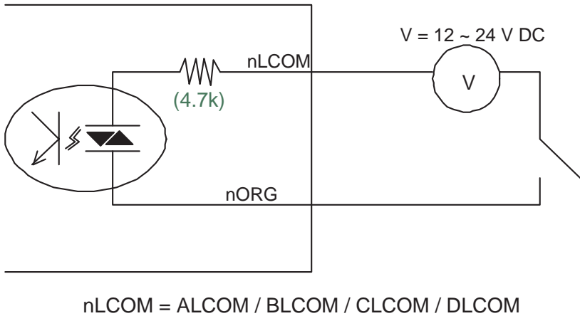
Figure 2.9: ORG Switch Test Configuration
