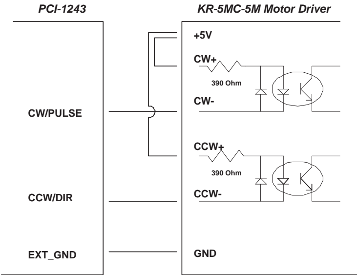
Figure 2.2: Output Connections Example
