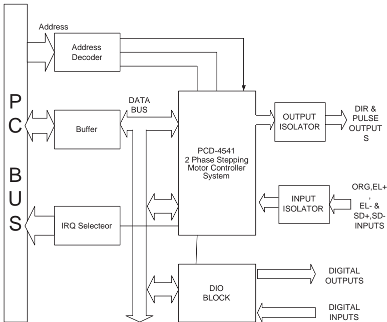
Figure 1.1: PCI-1243U 4-Axis Stepping Motor Control Card
