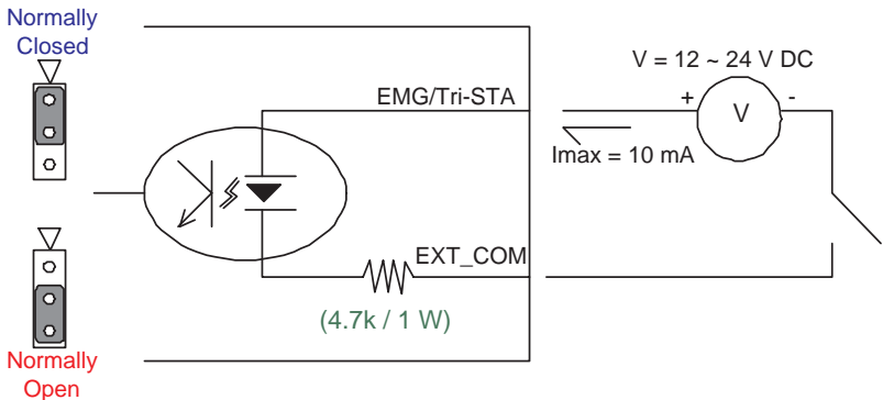
Figure 2.10: EMG / Tri_STA Test Configuration
