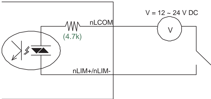
Figure 2.7: Lim Switch Test Configuration
