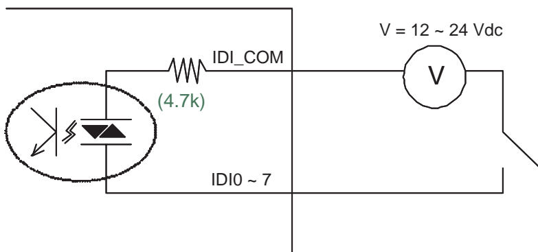
Figure 2.4: Isolated Digital Input Wiring Configuration
