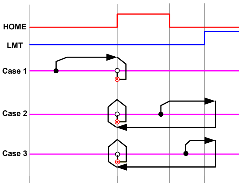
Figure C.4: Velocity Profile of Home Mode9
