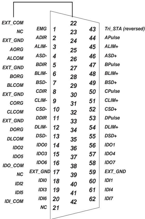
Figure 2.1: PCI-1243U Pin Assignment
