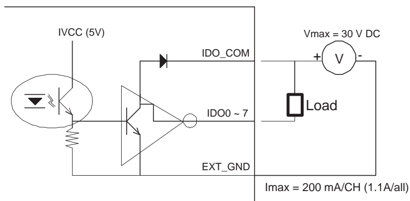
Figure 2.5: Isolated Digital Output Wiring Configuration
