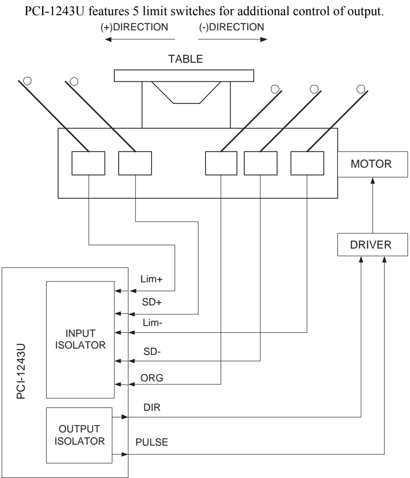
Figure 2.6: Limit Switches
