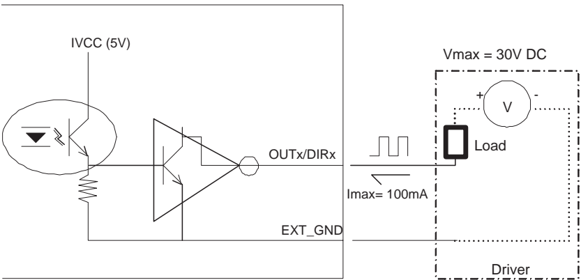
Figure 2.3: Pulse Output Test Configuration (Open Collector Type)
