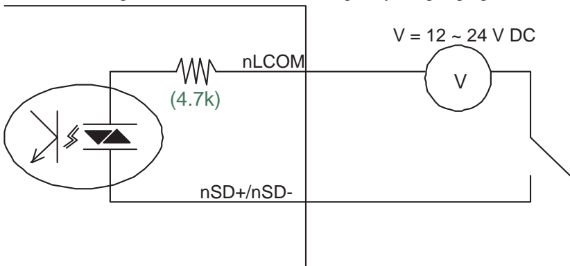
Figure 2.8: SD Switch Test Configuration
