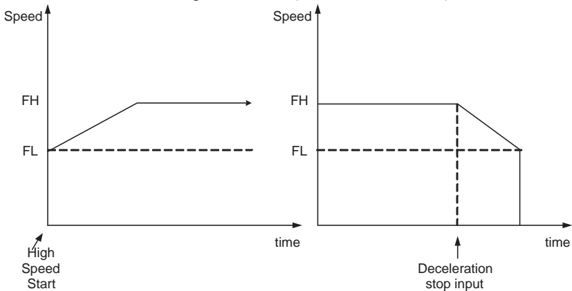
Figure 4.1: R4's Effect on Output Pulse Speed
