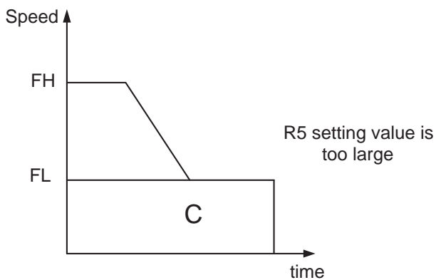
Figure 4.3: Setting the Ideal Ramping-Down Point
