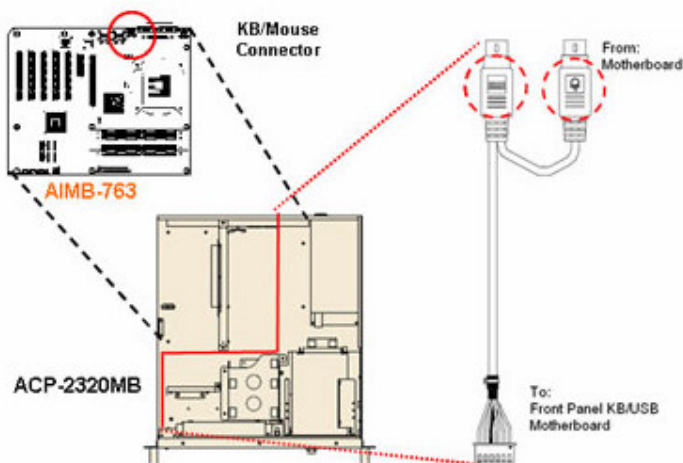
Fig.3 1700006917 connect with Keyboard/Mouse connector on motherboard and the KB/USB board on front panel
