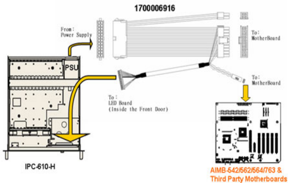
Fig.2 Assembly illustration of 1700006916
